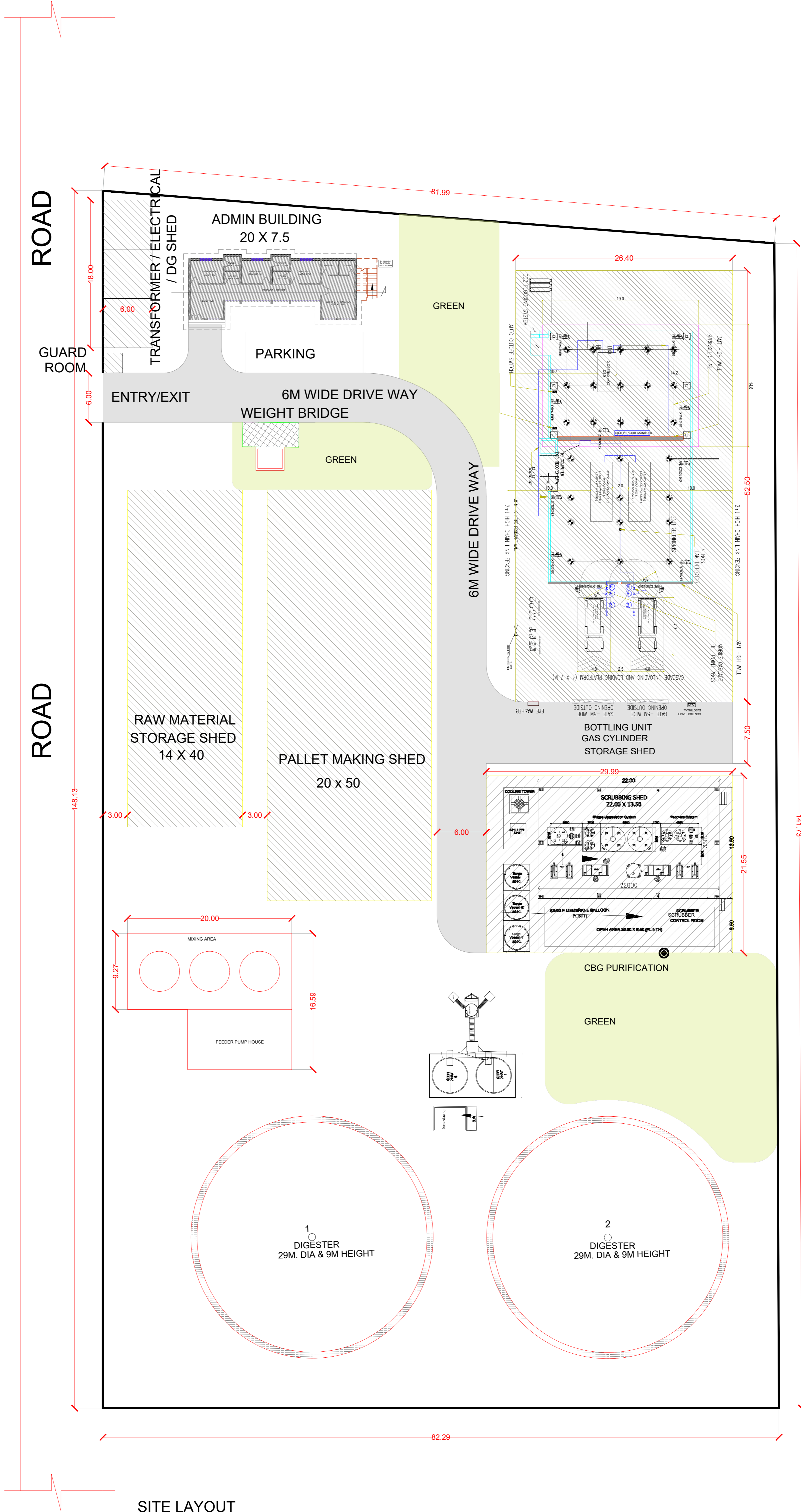
SITE LAYOUT
